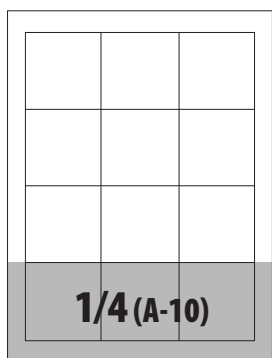
before trimming ..... 220x75 trimmed ..... 210x70 print area ..... 181x56
