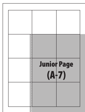
before trimming ..... 146x197 trimmed ..... 136x192 print area ..... 119x178
