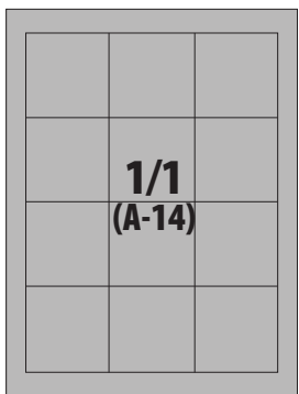
before trimming ..... 220x282 trimmed ..... 210x272 print area ..... 181x239
